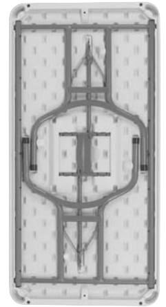
NEAT FOLDED UNDERSIDE SHOWING LEGS, CROSSBARS & STEEL CHANNELS
