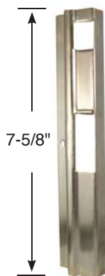
OLD STYLE RIGHT HAND LOCKING BAR FOR UPPER DOOR
