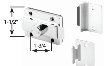
SLIDE LATCH & STRIKE & KEEPER SET
