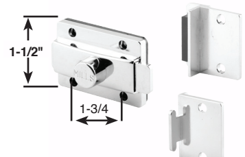
SLIDE LATCH & STRIKE & KEEPER SET
