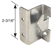
DOORSTOP Cat. #5580
